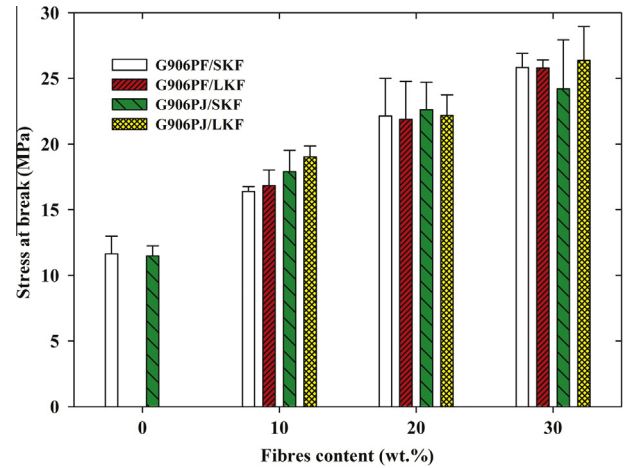
Fig. 7. Stress at break values of G906PF- and G906PJ-based composites with various amounts of SKF and LKF. (For interpretation of the references to colour in this figure legend, the reader is referred to the web version of this article.)
