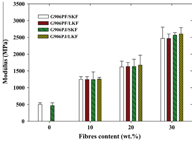
Fig. 5. Elastic modulus of G906PF- and G906PJ-based composites with various amounts of SKF and LKF. (For interpretation of the references to colour in this figure legend, the reader is referred to the web version of this article.)
