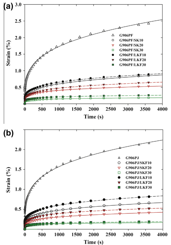
Fig. 11. Creep strain of (a) G906PF-based and (b) G906PJ-based composites with various amounts of SKF and LKF. (For interpretation of the references to colour in this figure legend, the reader is referred to the web version of this article.)
