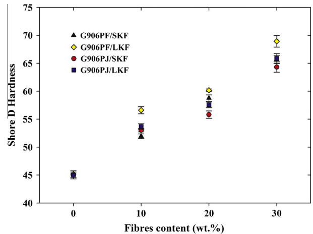
Fig. 10. Shore D hardness of G906PF- and G906PJ-based composites with various amounts of SKF and LKF. (For interpretation of the references to colour in this figure legend, the reader is referred to the web version of this article.)
