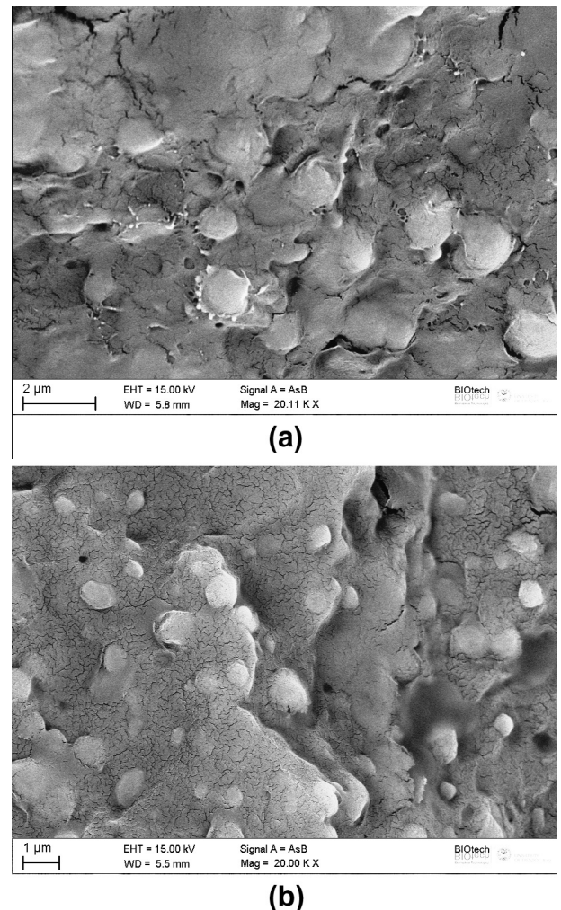
Fig. 1. FESEM micrographs of (a) G906PF and (b) G906PJ neat matrices.
