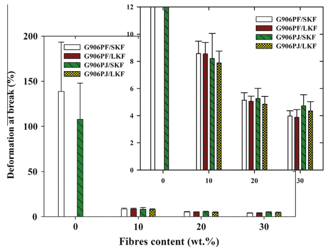
Fig. 8. Deformation at break values of G906PF- and G906PJ-based composites with various amounts of SKF and LKF. (For interpretation of the references to colour in this figure legend, the reader is referred to the web version of this article.)
