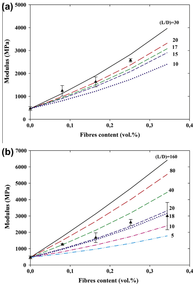
Fig. 6. Experimental (▲) and theoretical (lines) moduli values of G906PJ based composites reinforced by (a) SKF and (b) LKF. Predictions are based on the Halpin–Tsai model. (For interpretation of the references to colour in this figure legend, the reader is referred to the web version of this article.)
