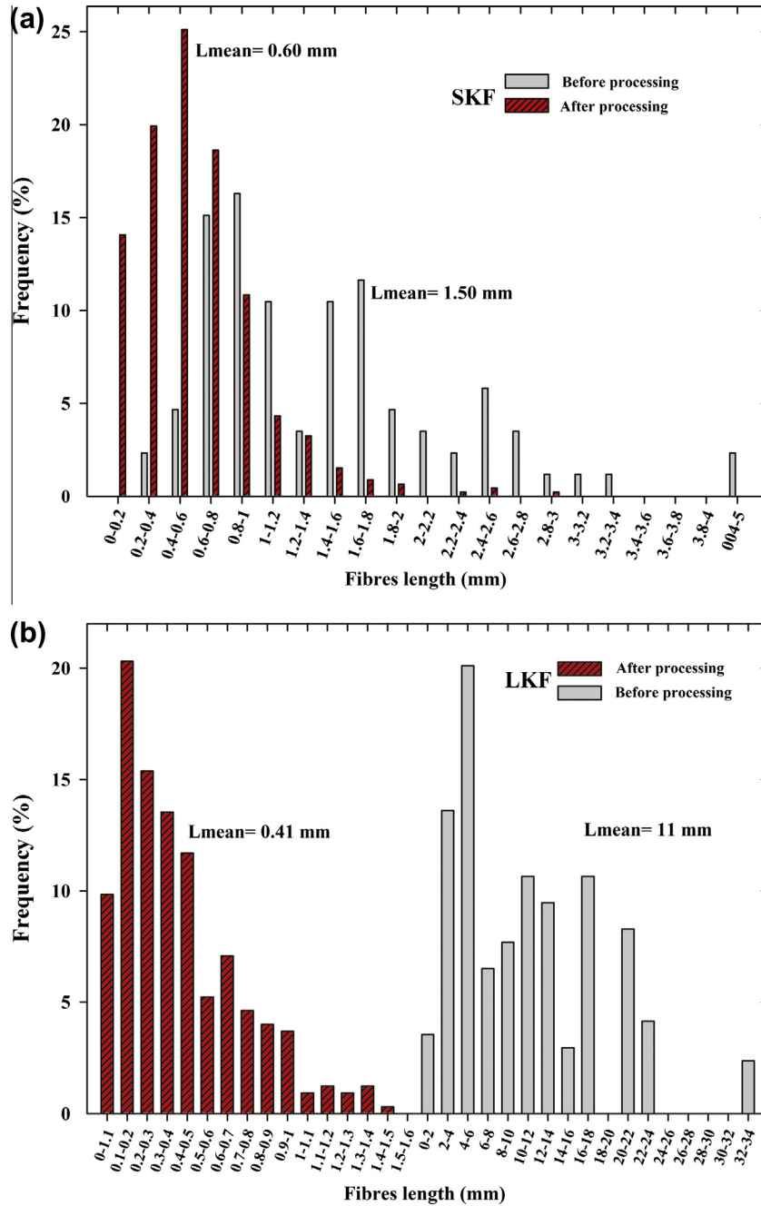
Fig. 3. Histograms of length distribution for (a) SKF and (b) LKF, before and after processing. (For interpretation of the references to colour in this figure legend, the reader is referred to the web version of this article.)
