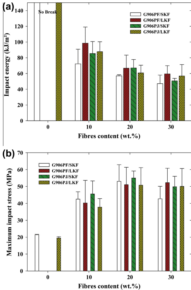
Fig. 9. (a) Impact energy and (b) maximum impact stress of G906PF- and G906PJ-based composites with various amounts of SKF and LKF. (For interpretation of the references to colour in this figure legend, the reader is referred to the web version of this article.)
