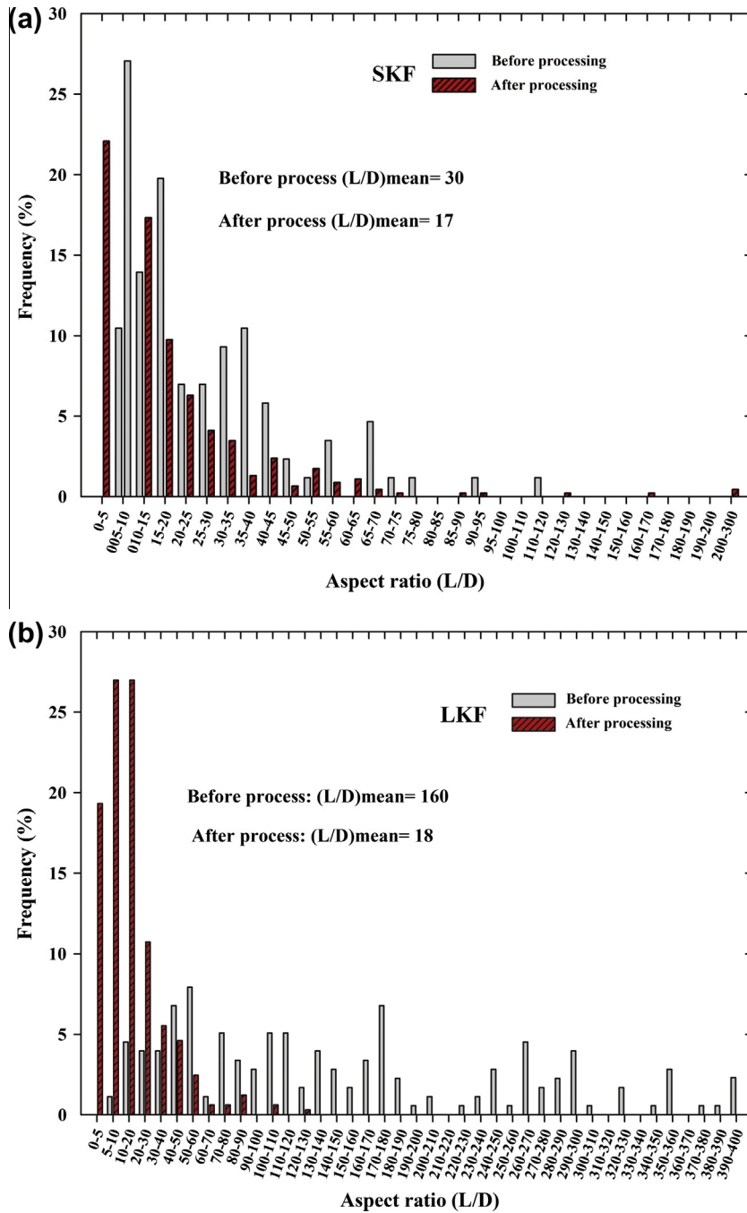
Fig. 4. Histograms of aspect ratio distribution for (a) SKF and (b) LKF, before and after processing. (For interpretation of the references to colour in this figure legend, the reader is referred to the web version of this article.)
