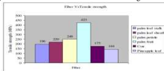
Fig 2: Tensile strength of palm fibers and other fiber.
