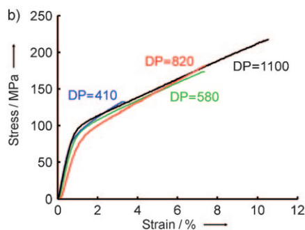
Figure 10. a) Transparent MFC film made from carboxymethylated MFC (courtesy: David Placket and Istvan Siro, Risø DTU, Roskilde). b) Typical stress–strain curves for MFC films prepared from pulps with various degrees of polymerization. [1d]
