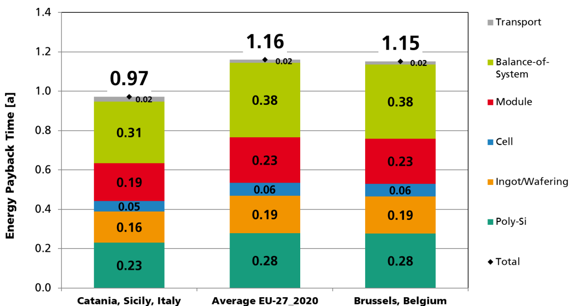
Figure 29: Calculated energy payback times of PV power plants for European production and operating sites [ISE10], data: Lorenz Friedrich
