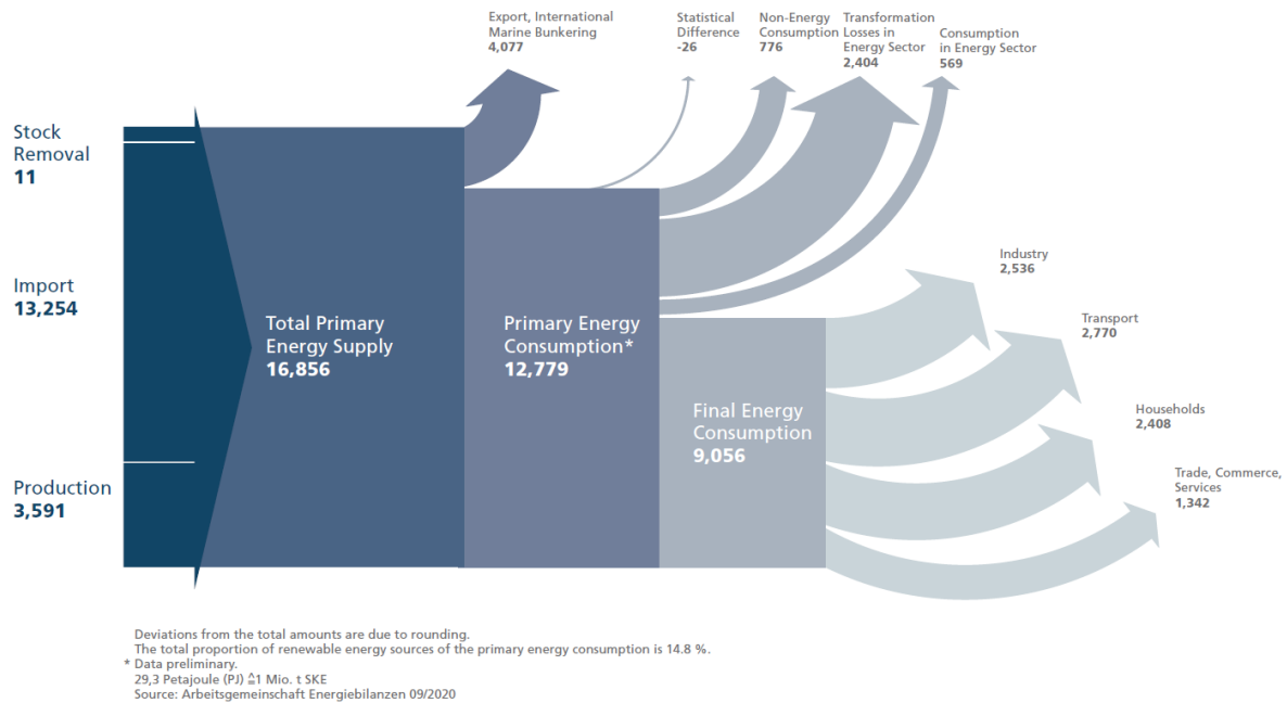
Figure 42: Energy flow diagram 2019 for Germany in petajoules [AGEB].
