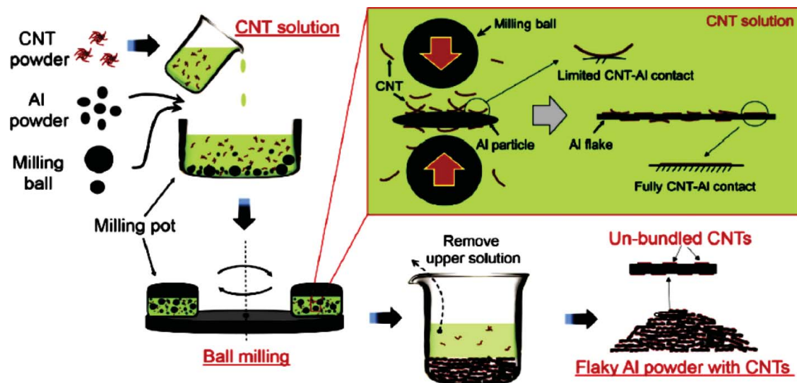
Figure 3. Diagram of Solution Ball Milling (SBM) for the uniform dispersion of CNTs. (© Elsevier Limited. Reprinted with permission from Chen et al. 81 Permission to reuse must be obtained from the rightsholder.)
