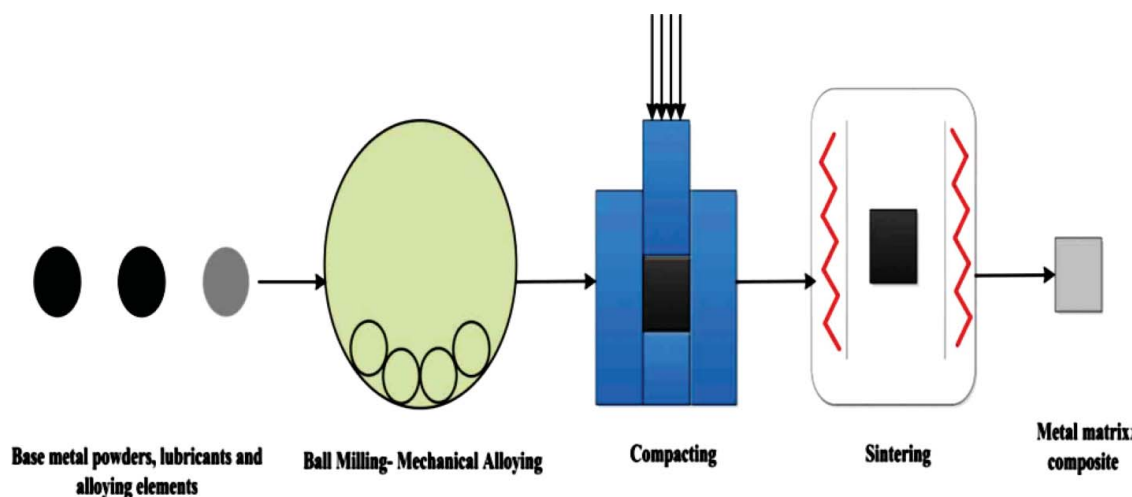
Figure 2. Schematic process of P/M technology. (© Taylor & Francis. Reprinted with permission from Munir et al. 66 Permission to reuse must be obtained from the rightsholder.)
