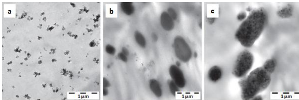
Figure 7. Dispersion of (a) boehmite alumina (BA); (b) polyurethane (PU)); (c) BA + PU in a polyoxymethylene (POM) based system based on transmission electron microscopy (TEM) investigations [28]. Note (a) the fine dispersion of BA; (b) the micron range dispersion of PU (the usual requirement for impact modifier); (c) the BA embedding in the PU phase.
