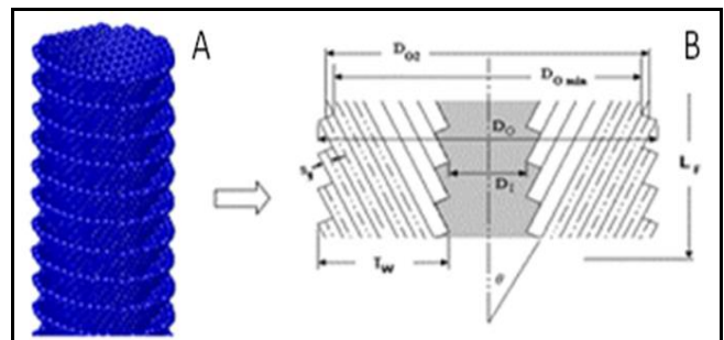
Figure 5 A) Stacked-cup CNF. B) Cross section view showing the internal structure of a CNF stacked-cup (Source: Pyrograf).
