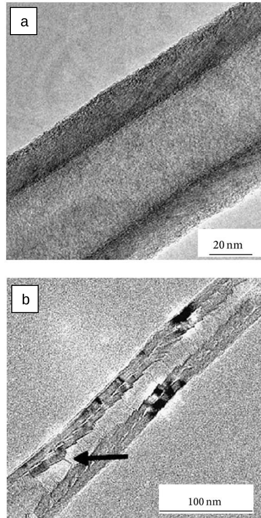
Figure 4 CNF TEM micrograph displaying (a) a single layer, and (b) a double layer [71, 72]
