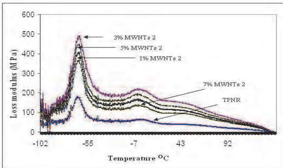
Fig. 8. Loss modulus of TPNR and TPNR/MWNTs 2 nanocomposites.
