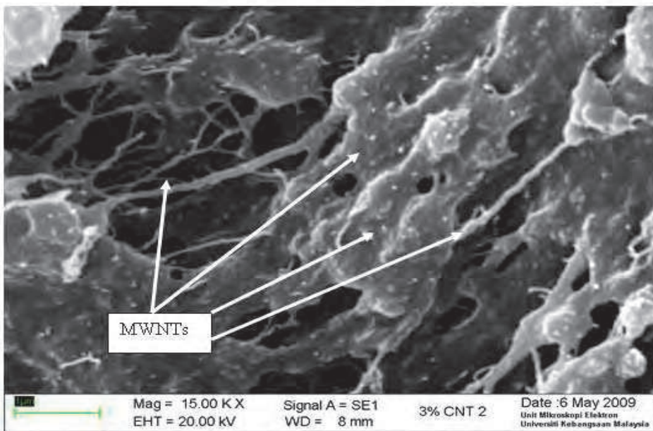
Fig. 25. SEM micrograph of TPNR with 3% MWNTs 2.
