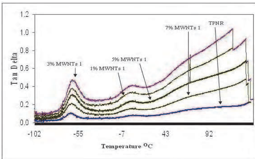
Fig. 9. Tan delta of TPNR and TPNR/MWNTs 1 nanocomposites.
