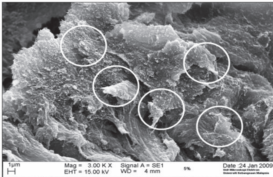
Fig. 22. SEM micrograph of TPNR with 5% MWNTs 1.
