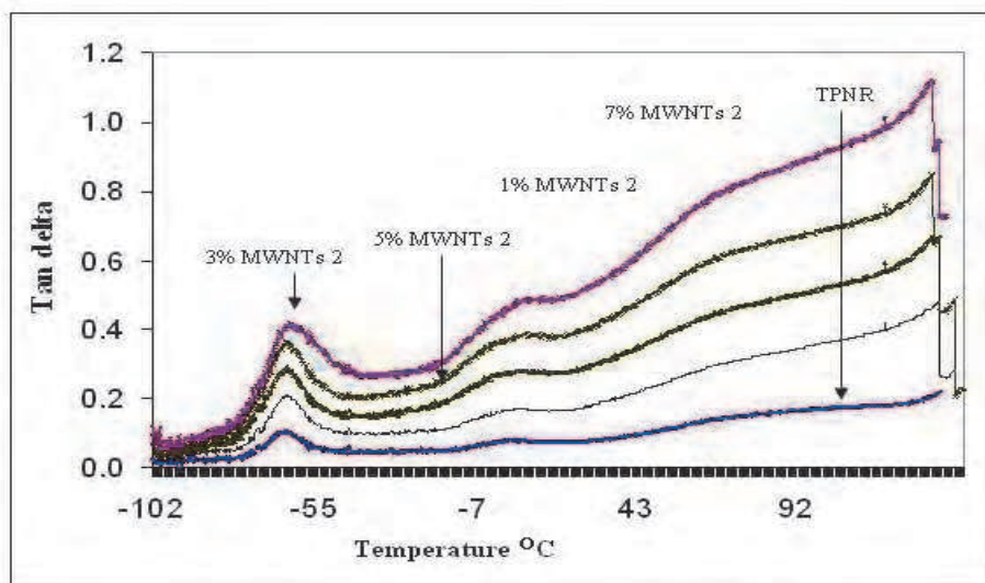
Fig. 10. Tan delta of TPNR and TPNR/MWNTs 2 nanocomposites.
