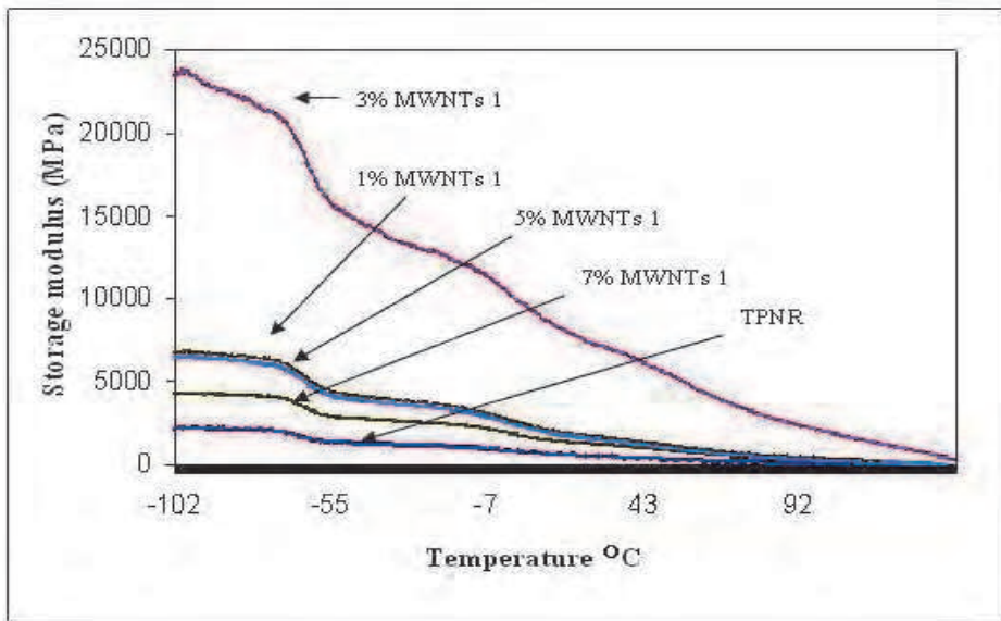
Fig. 5. Storage modulus of TPNR and TPNR/MWNTs 1 nanocomposites.
