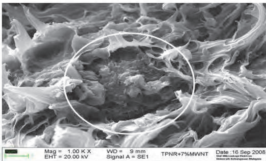
Fig. 23. SEM micrograph of TPNR with 7% MWNTs 1.
