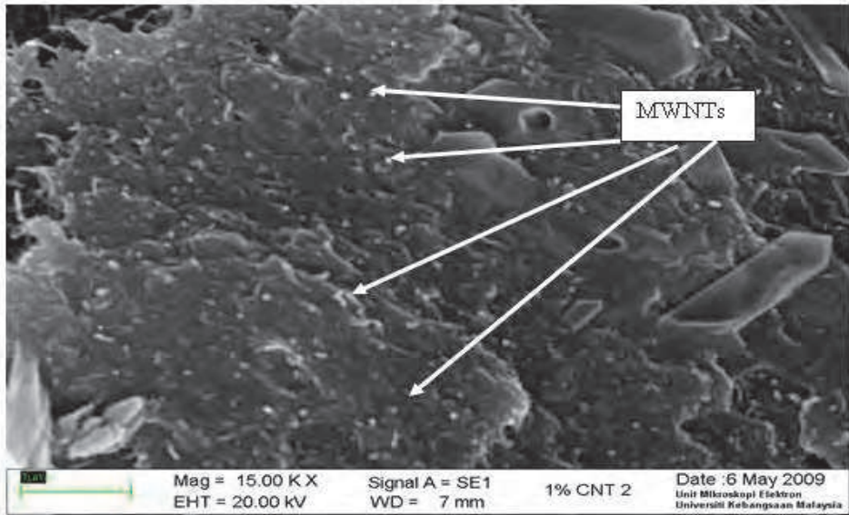
Fig. 24. SEM micrograph of TPNR with 1% MWNTs 2.
