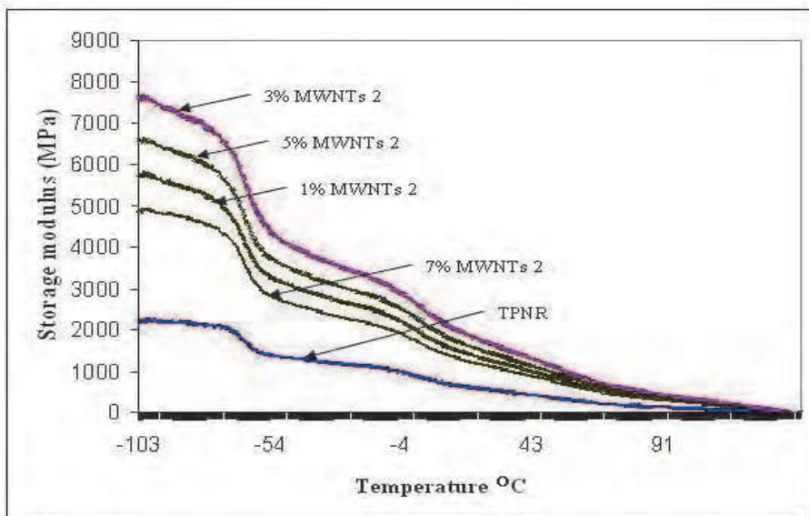
Fig. 6. Storage modulus of TPNR and TPNR/MWNTs 2 nanocomposites.
