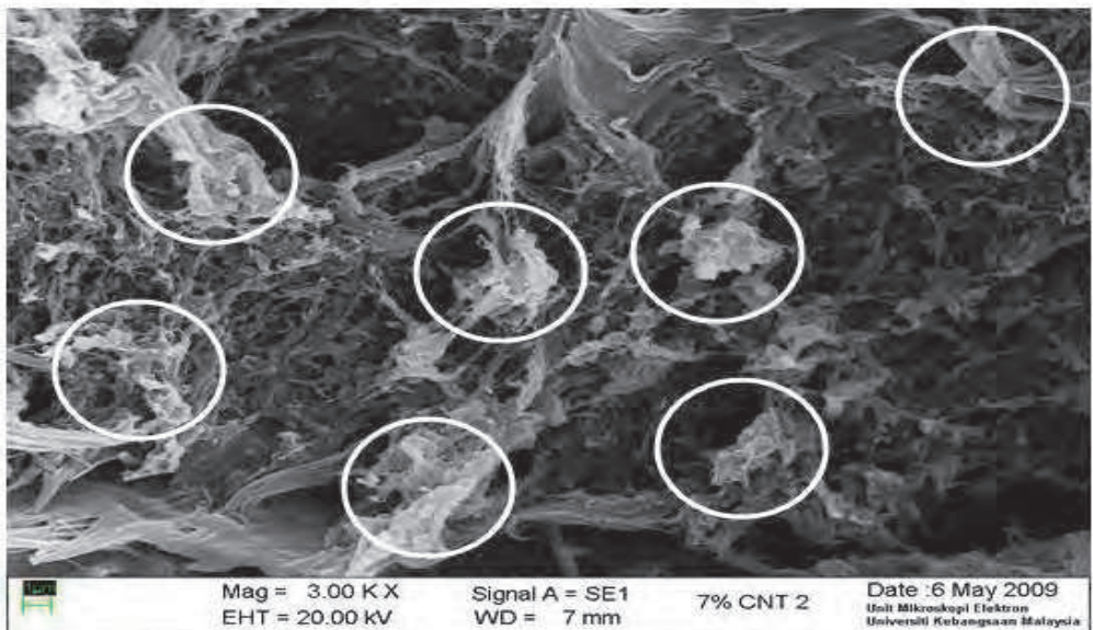
Fig. 27. SEM micrograph of TPNR with 7% MWNTs 2.
