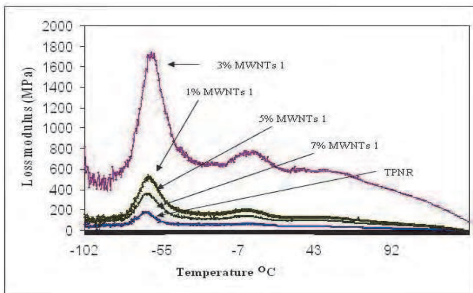
Fig. 7. Loss modulus of TPNR and TPNR/MWNTs 1 nanocomposites.
